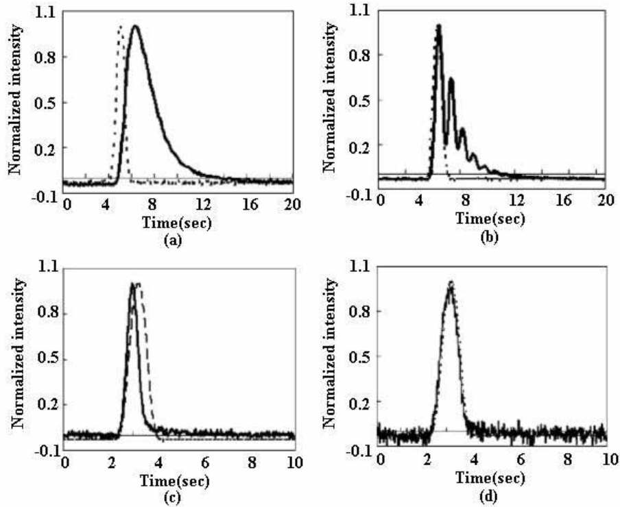
Fig. 4. Experimental results showing the group velocity variation of the signal output with setting the separation of the gain doublet to (a) 0Hz, (b) 1Hz, (c) 2Hz, and (d) 4Hz. Dashed line indicates reference, solid line indicates signal output
