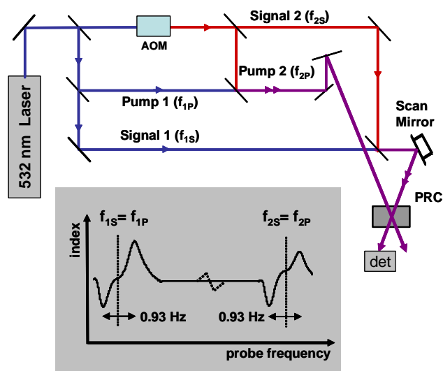
Fig. 5. (Top) Experimental set-up for measuring the dispersion profile directly. (Bottom) Observed dispersion profile centered around two pump frequencies. See text for additional details.
