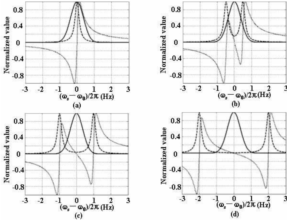
Fig. 1. Numerical, normalized plots of S(\omega) , the Fourier transform of the input pulse (solid line), \Gamma_{in} (dashed line), and \Gamma_{ph} (dotted line). The input pulse is assumed to be of the form \exp(-t^2/t_0^2) . For these plots, we have used for t_0=0.6\text{sec} , \Gamma_0 d=6 and \tau_1 = \tau_2 \equiv \tau_M = 1.1\text{sec} . The four sets are for four different gain separations, 2\Delta\omega (a) 0Hz, (b) 1Hz, (c) 2Hz, (d) 4Hz
