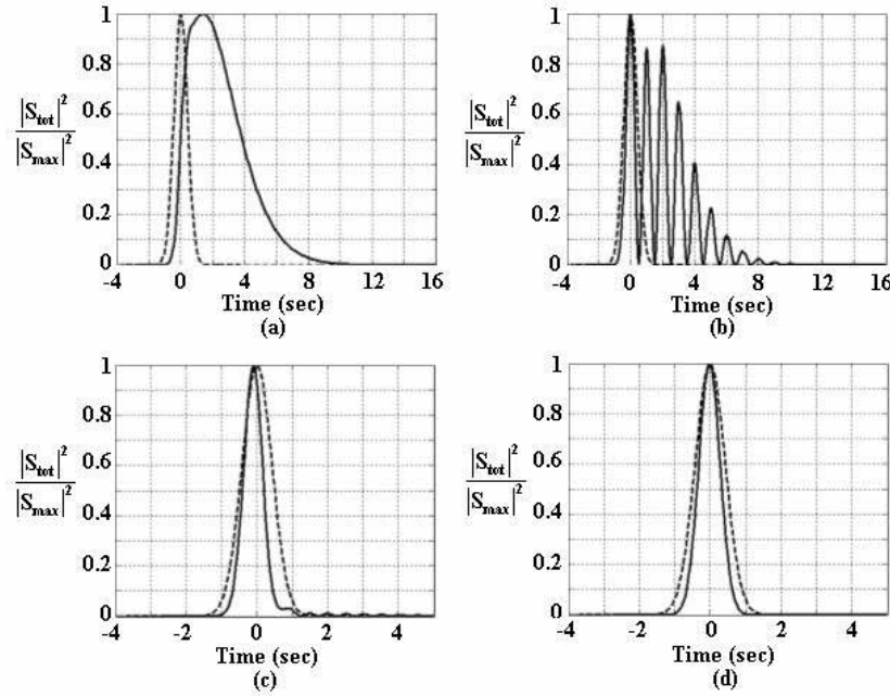
Fig. 2. Simulated output signal for the Gaussian input of \exp(-t^2/t_0^2) for the same parameters as set in Fig. 1. The frequency difference between the gains is given as (a) 0Hz, (b) 1Hz, (c) 2Hz, and (d) 4Hz. Dashed line indicates reference, solid line indicates signal output.
