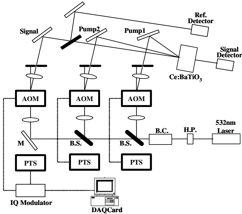
Fig. 3. Schematic diagram of the experimental set-up; AOM : Acousto-optic modulator, B.S: Beam Splitter, B.C : Beam Collimator, H.P: Half-wave plate, M: Mirror, PTS : Frequency synthesizer, Pump1: f_L+110\text{MHz}+4\text{Hz}+\Delta\omega , Pump2: f_L+110\text{MHz}+4\text{Hz}-\Delta\omega , Probe : Gaussian pulse with the carrier frequency of f_L+110\text{MHz}+4\text{Hz}
